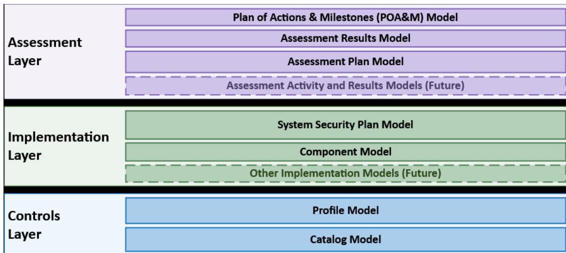
Figure 2. Layers and Models in OSCAL.
