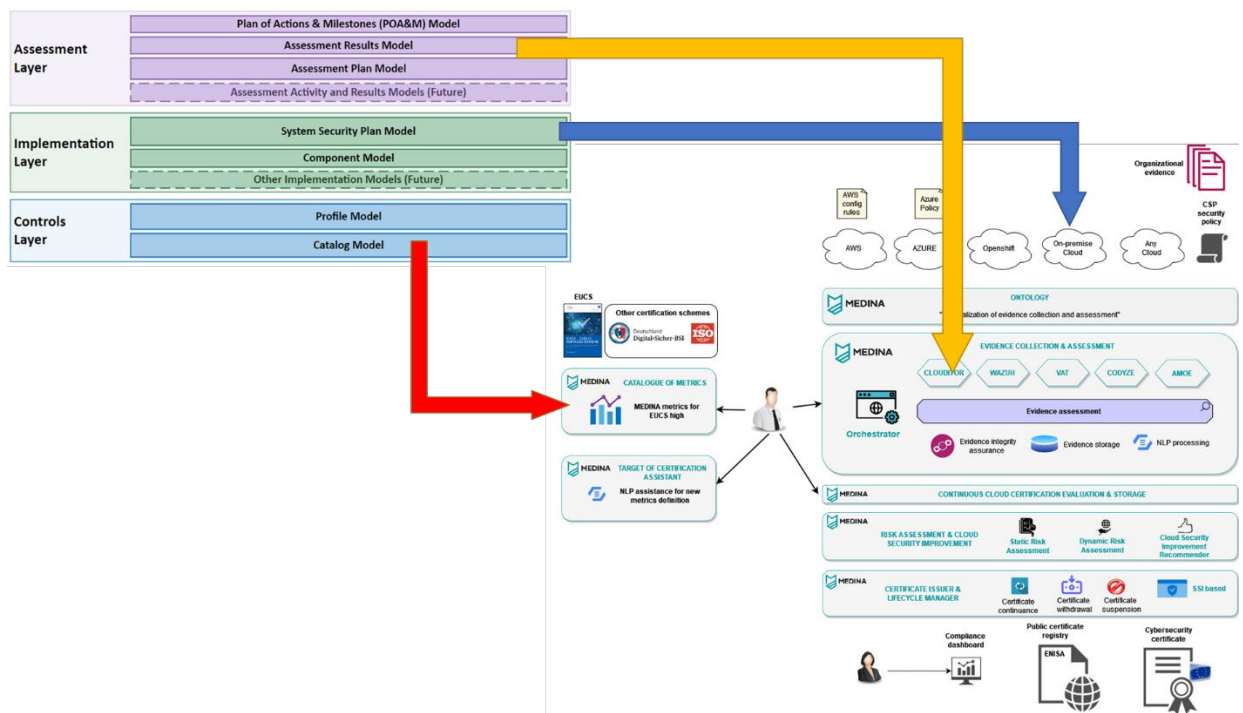
Figure 4. Leveraging OSCAL in the MEDINA framework.
